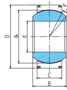
GE(H)···XT
