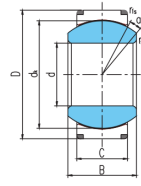
GEC(H)...XT
