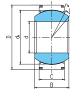
GEC(H)...XT-2RS
